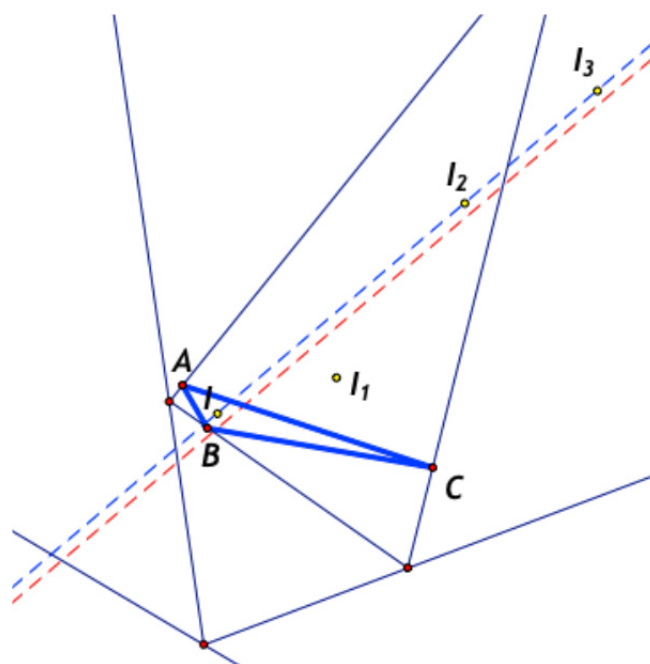
FIGURE 5: Counter-example to Conjecture 2.
