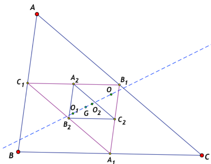
FIGURE 3: Iteration of circumcentres.
