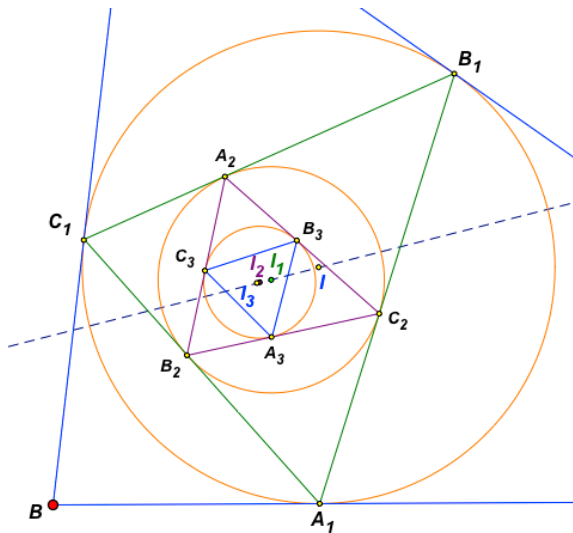
FIGURE 1: Investigation 1 – Iteration of tangent points of incircle.
