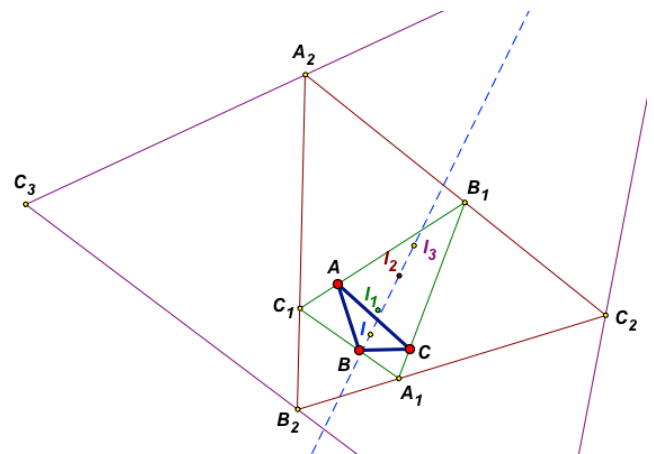
FIGURE 2: Investigation 2 – Iteration of excentres.
